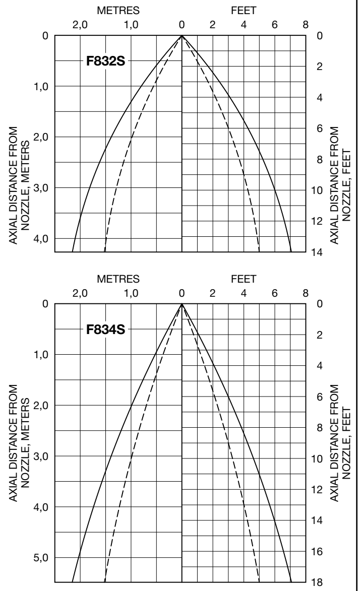
GRAPH A (1 OF 2) WATER DISTRIBUTION DESIGN DATA
